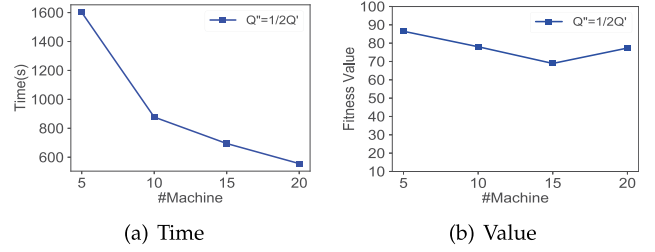
Fig. 9. Fixed number of partitions per node.
