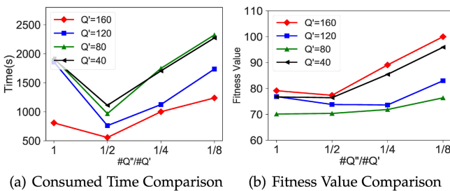
Fig. 8. Impact analysis of partition configuration.
