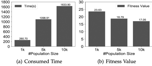
Fig. 7. The impact of population size setting.
