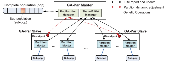
Fig. 4. The architecture and module interactions in GA-Par.
