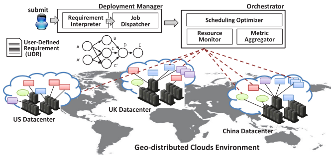
Fig. 2. Microservice orchestration in a geo-distributed cloud environment.
