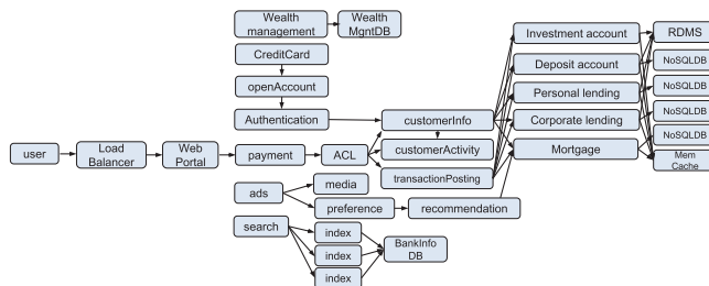
Fig. 1. e-banking microservices (a representative case [15]).
