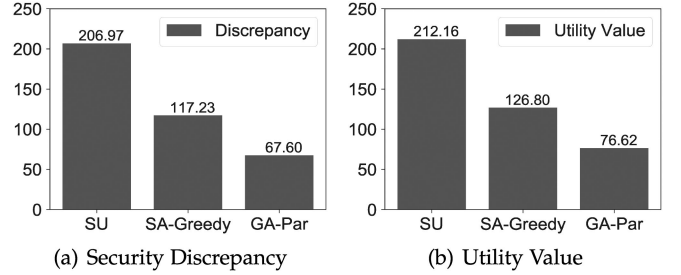
Fig. 5. Security enhancement effects by different methods.
